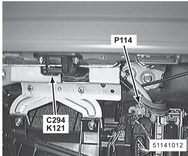
185. behind RH side of fascia K121 Heated Front Screen Relay P114 Heated Front Screen Fuse Block C294 (4-W)
