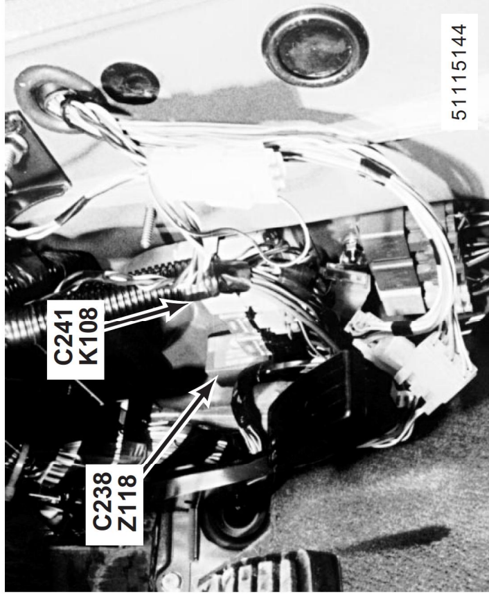
152. behind RH footwell trim panel (MFI-V8 shown; others similar)
