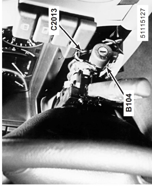
105. top of steering column B104 Column Switch Illumination C2013 (4-B)
