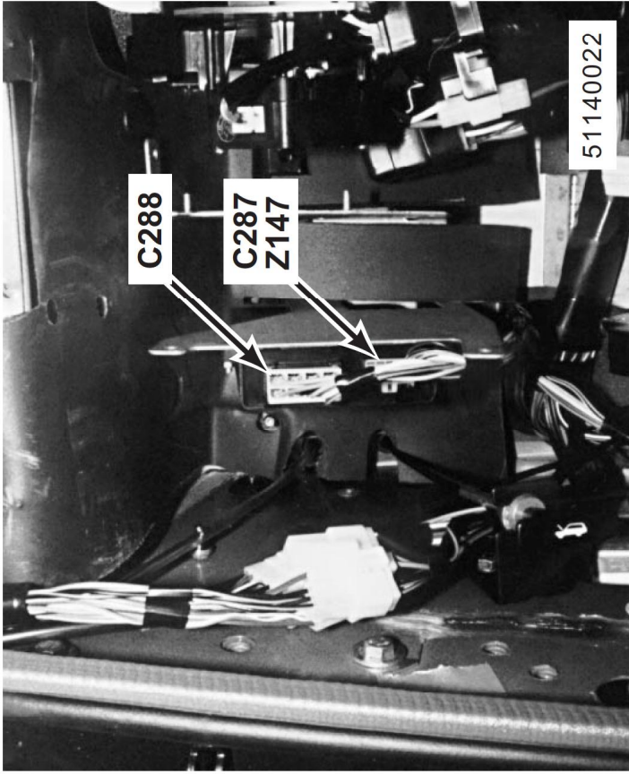
101. behind LH side of fascia Z147 Window Lift ECU C287 (10-W) C288 (8-W)
