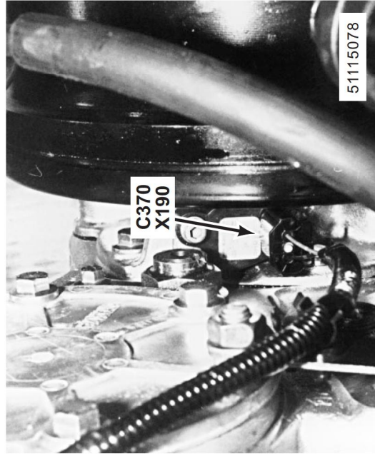
81. LH side of transfer box X190 Vehicle Speed Sensor C370 (3-B)
