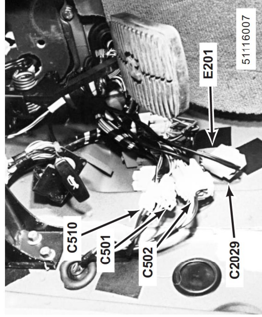
84. behind LH footwell trim panel E201 C501 (2-W) C502 (13-W) C510 (2-W) C2029 (6-W)
