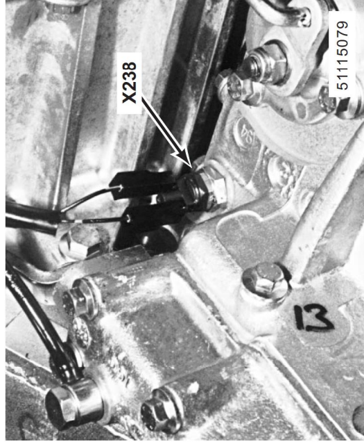
82. top RH side of transfer box X238 Differential Lock Switch
