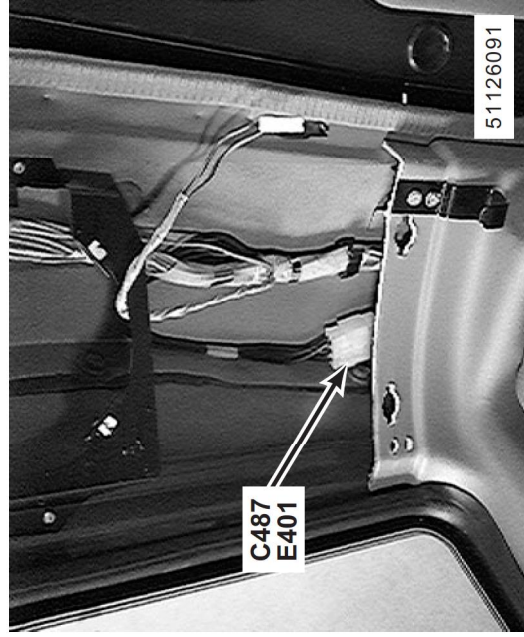
243. RH rear of luggage compartment behind trim panel C487 (6-W) E401
