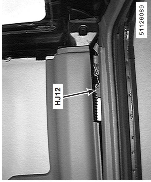
242. LH rear of roof behind trim panel HJ12 (20-G)
