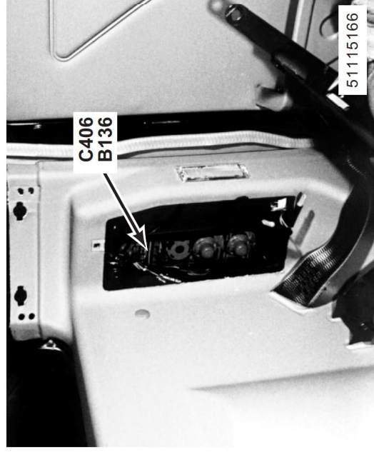
244. RH rear of luggage compartment behind trim panel B136 Right Rear Lamp Assembly C406 (6-W)
