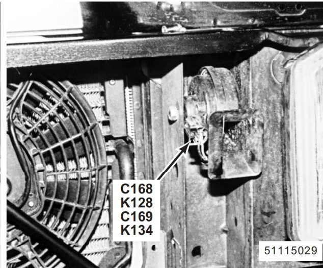
40. LH front of vehicle (RH similar) K128 Left Horn K134 Right Horn C168 (2-B) (Left) C169 (2-B) (Right)
