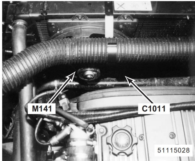
39. front of engine compartment (MFI-T16 without Air Conditioning) M141 Cooling Fan Motor 1 C1011 (2-W)
