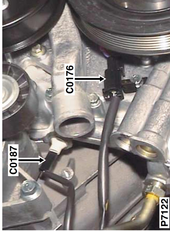
Description: Switch-Oil pressure - V8 Location: Lower front of engine - RH side
