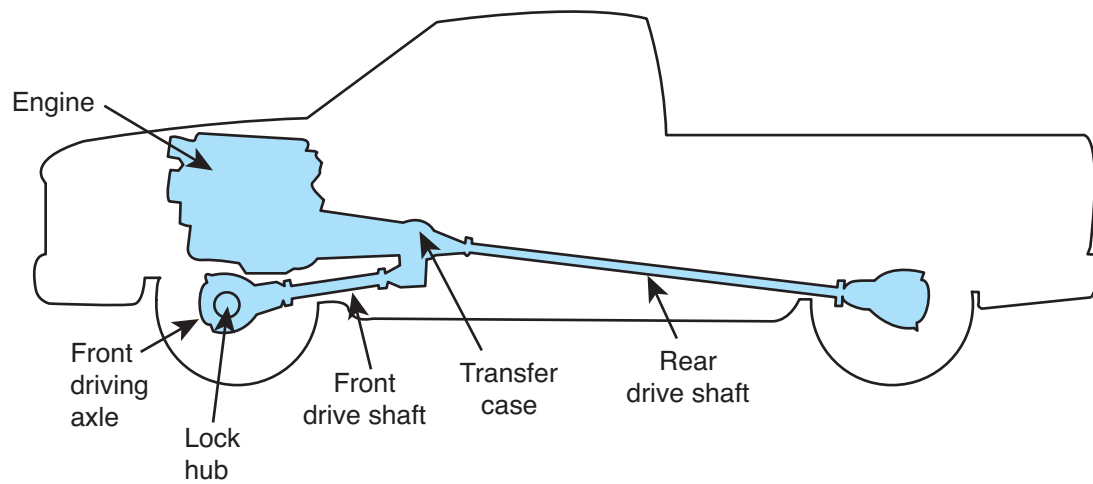
Figure 6-4 4WD truck with two drive shafts.
