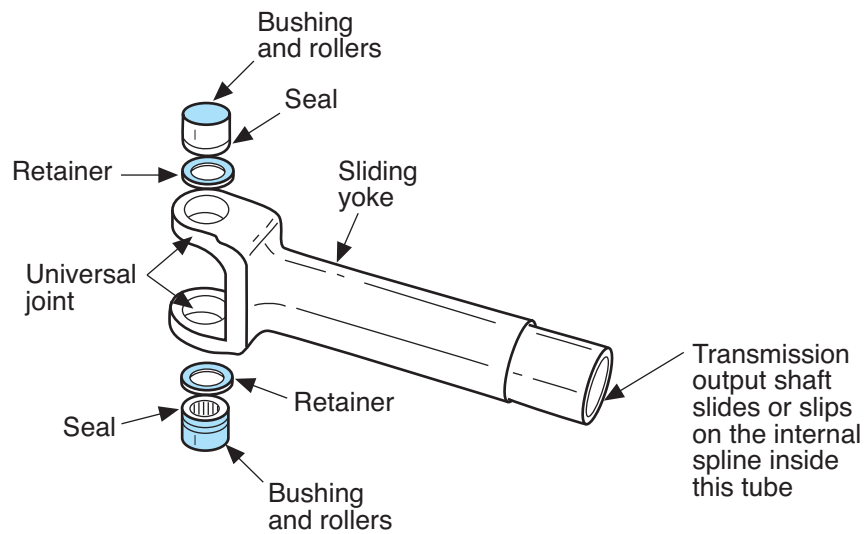
Figure 6-25 Typical slip joint assembly.
