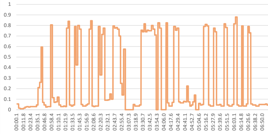
Oxygen Sensor Voltage Bank 1 - Sensor 1
