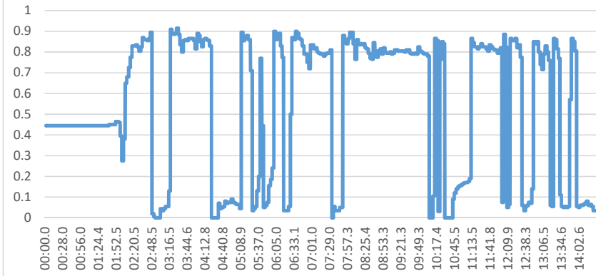
Oxygen Sensor Voltage Bank 1 - Sensor 2
