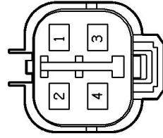
Description: Sensor-Heated oxygen (HO2S)-Front-LH Location: Rear LH side of engine
