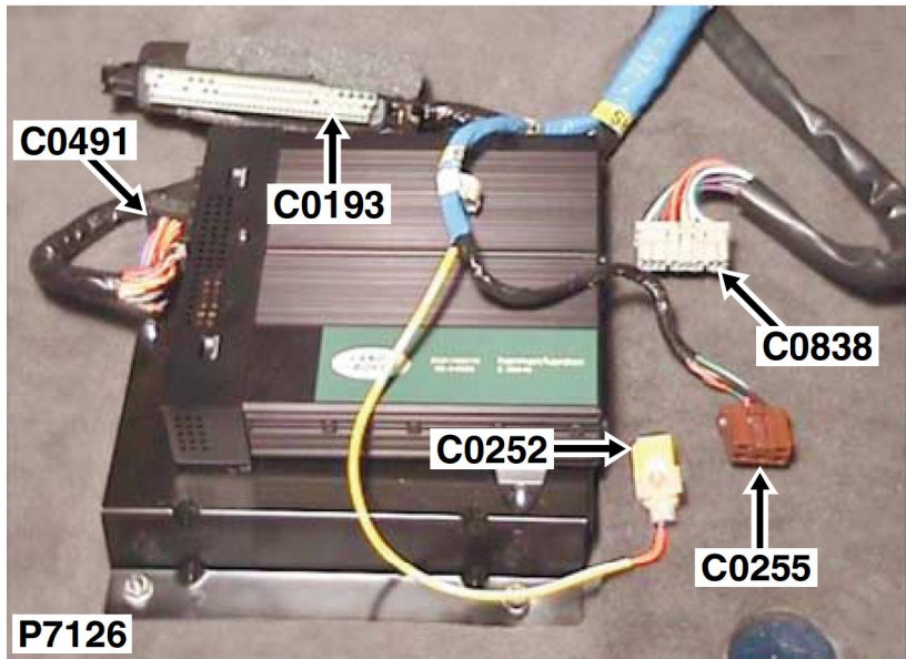
Description: Amplifier-Power-ICE Location: Beneath LH seat
