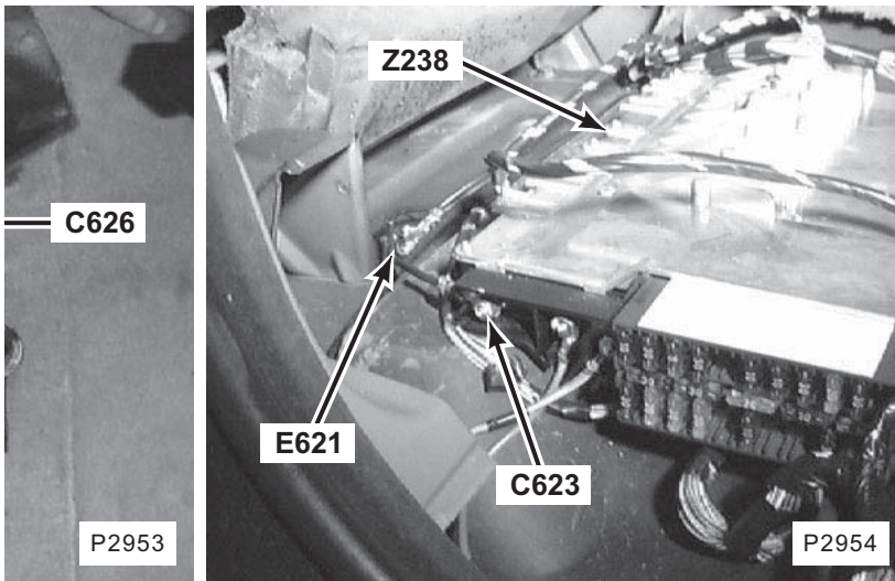
200. beneath RH front seat Z238 Body Electrical Control Module (BECM) C623 E621
