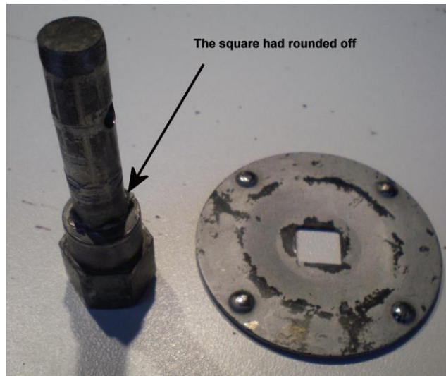
Figure 3 The Damaged Shaft
