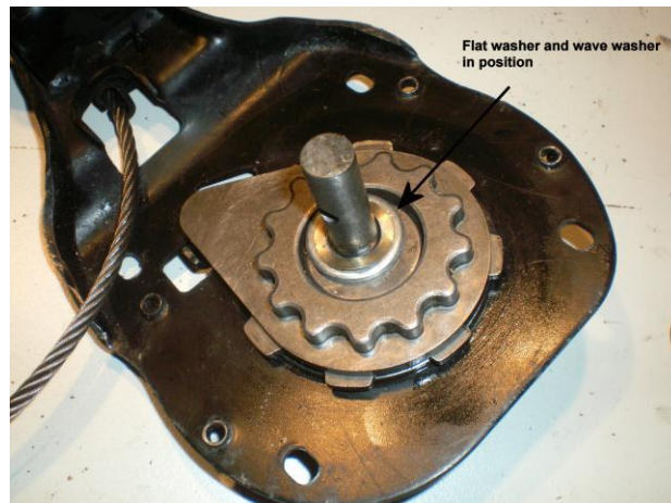
Figure 7 Flat Washer and Wave Washer in Position
