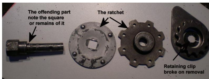
Figure 2 Dismantled Shaft and Clutch Ratchet
