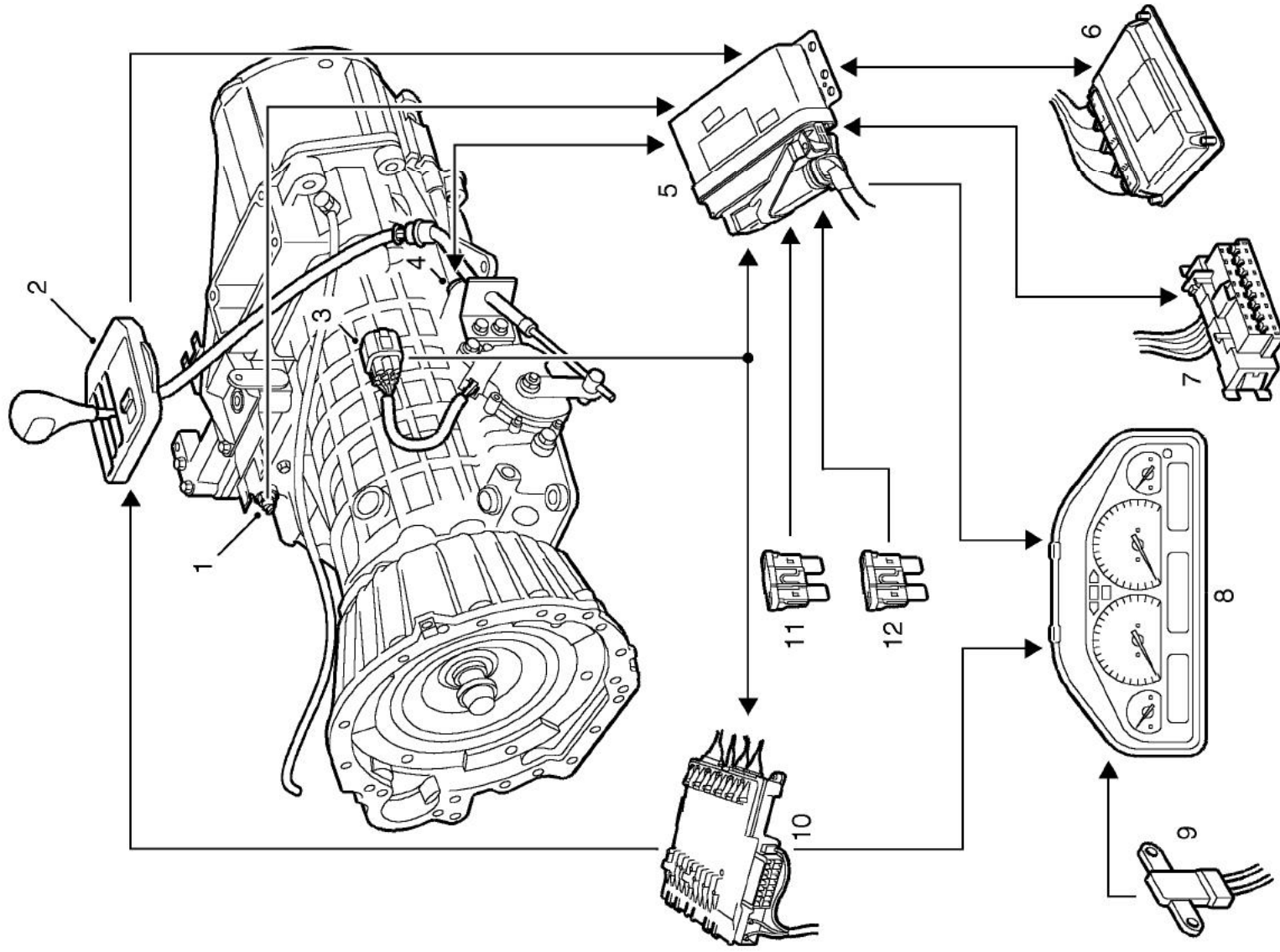
Electronic Automatic Transmission control schematic
