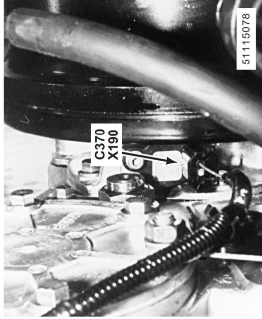
117. LH side of transfer box X190 Vehicle Speed Sensor C370 (3-B)
