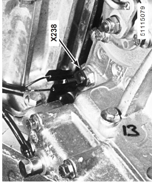
118. top RH side of transfer box X238 Differential Lock Switch
