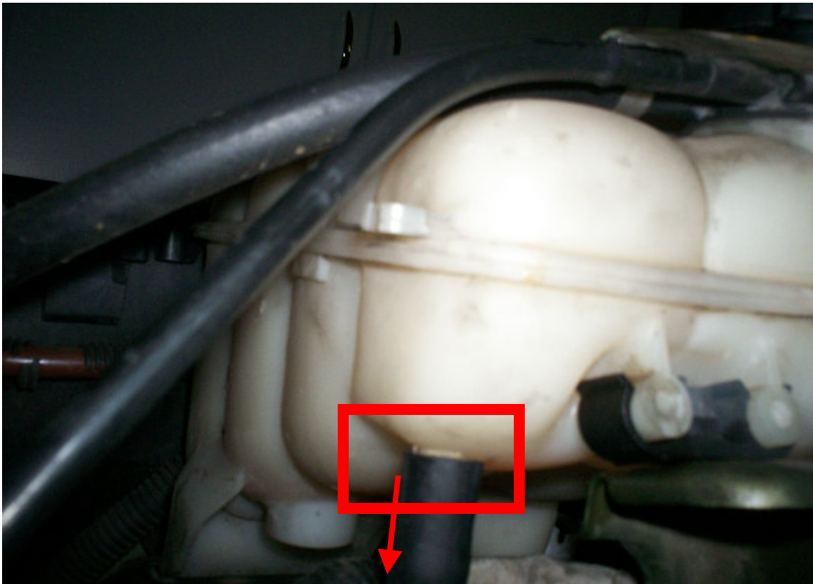
Coolant flows down from edge of hose
