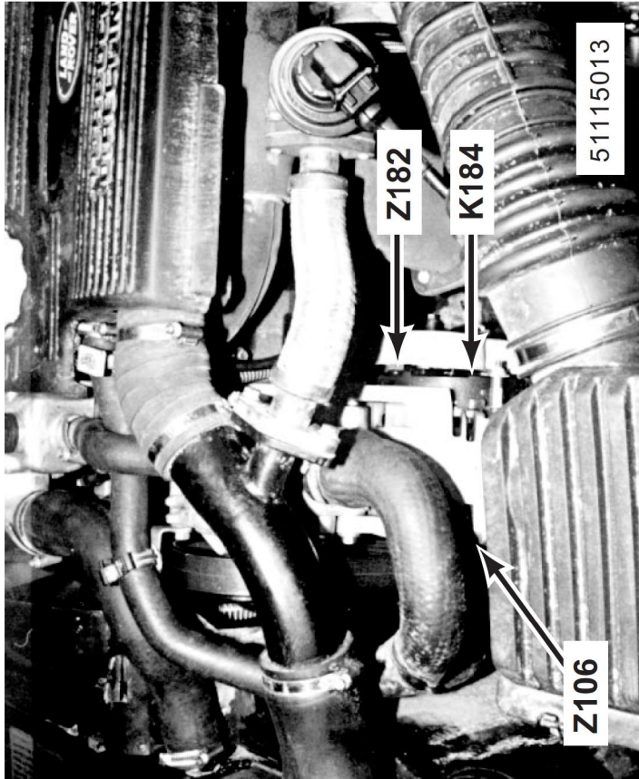
15. lower LH side of engine 300Tdi K184 Phase Tap Resistor Z182 Generator Suppression Capacitor Z106 Generator
