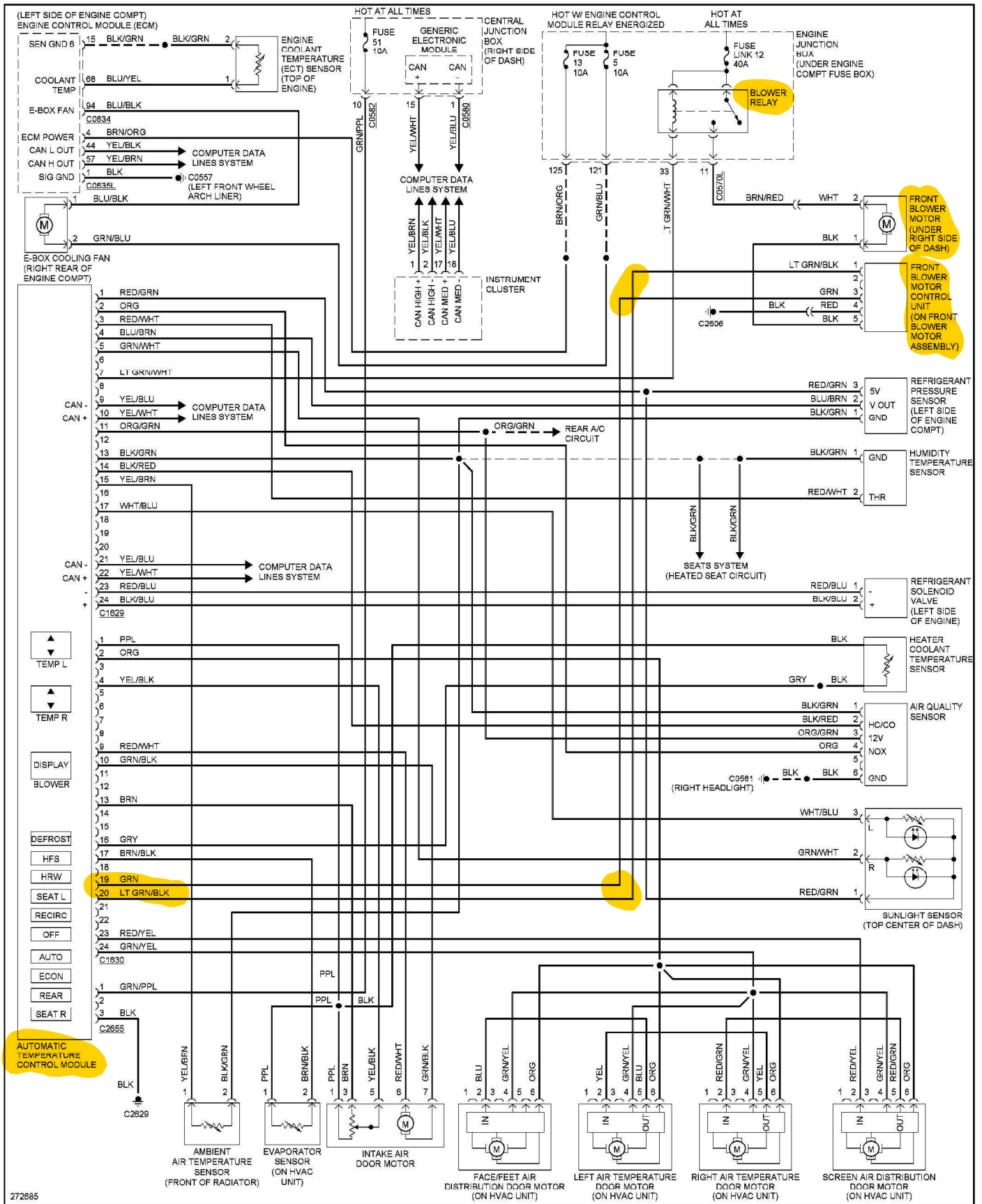
Fig. 1: Automatic A/C Circuit, W/ TSD
