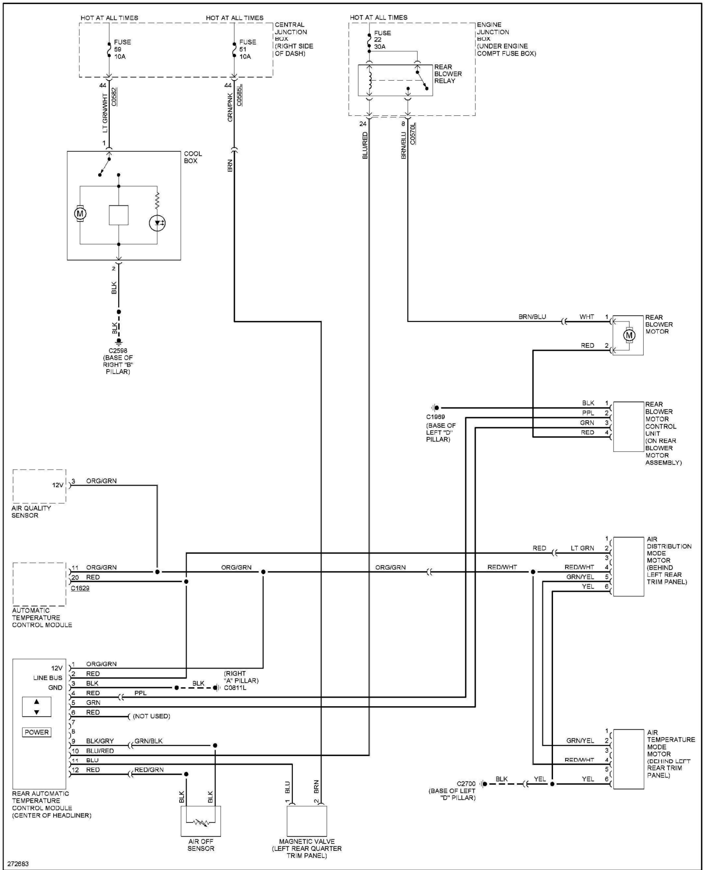
Fig. 3: Rear A/C Circuit
